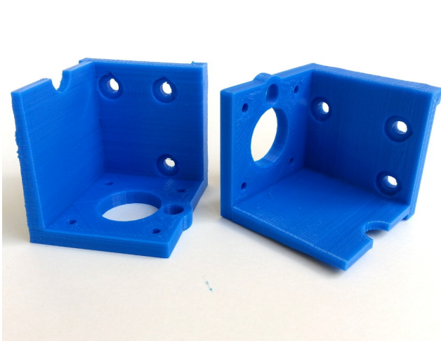
Z Motor mount (1 pair)
